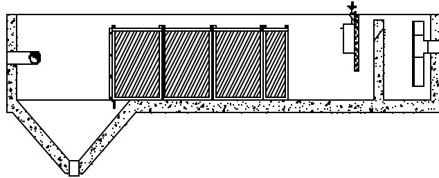
HOPPER BOTTOM DESIGN
